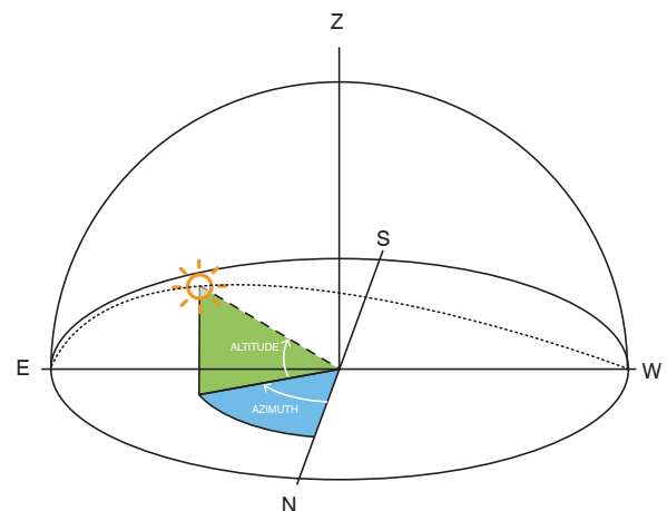
Azimuth and Altitude Angles
